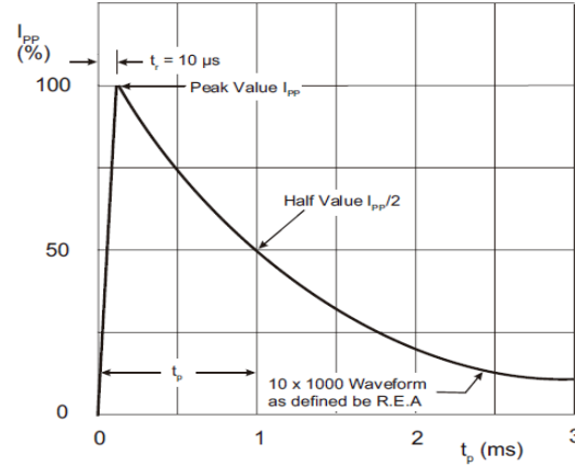
Figure2. Pulse waveform
